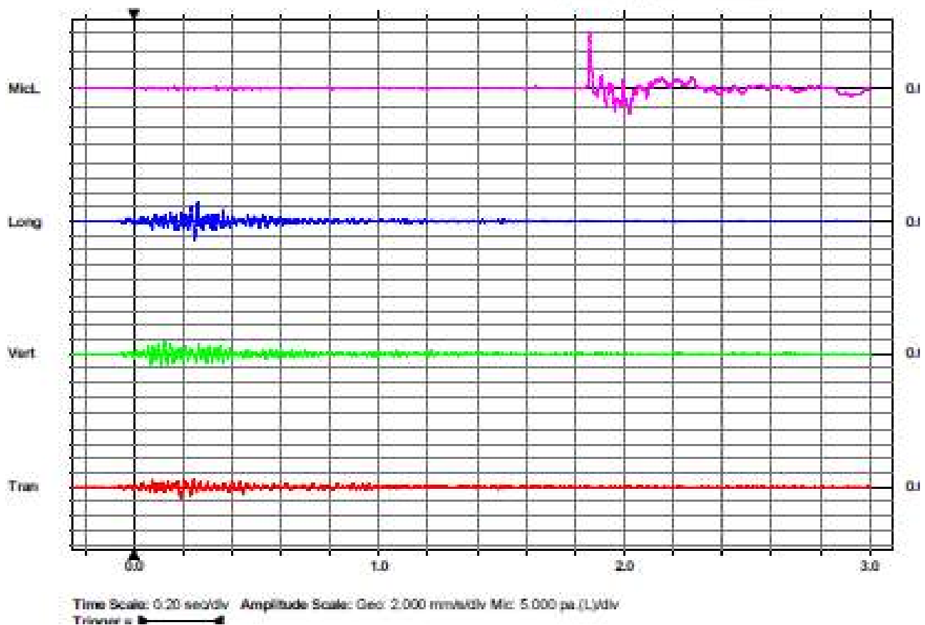
A sample of ground vibration monitoring report
